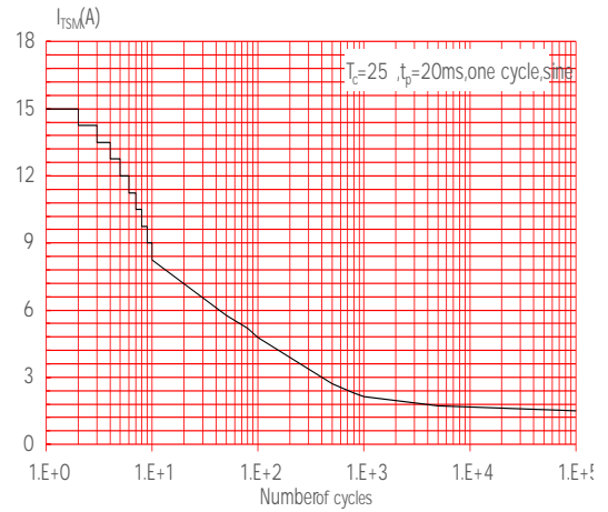
FIG.6: Non-repetitive surge peak onstate current for a sinusoidal pulse with width t_p < 20ms , and corresponding value of di/dt < 60A/\mu s
