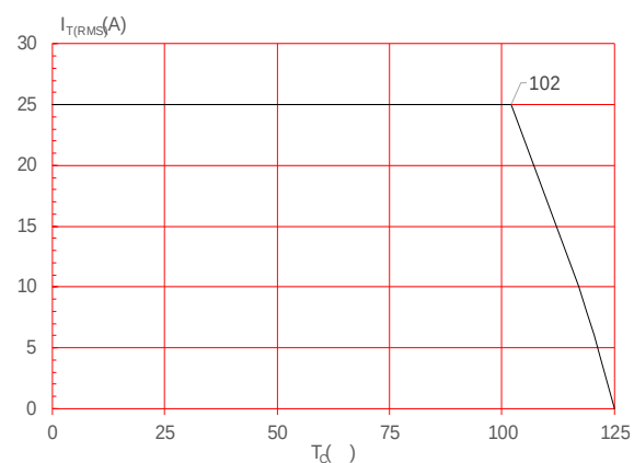
FIG.4: On-state characteristics
